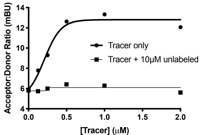
NL-PHKG2 Tracer 10-7600 CTx-0294885 EC50
