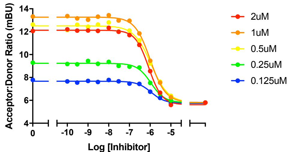
NL-PHKG2 Tracer 10-7600 CTx-0294885
